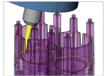
5軸CAM
